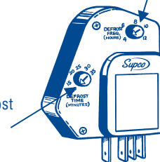
Dial control for setting Defrost frequency from 4 to 12 hours.
