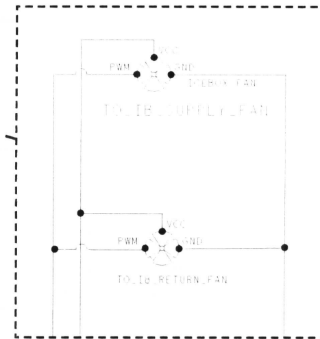
MODIFIED TECH SHEET AFTER KIT INSTALLATION (SCHEMATIC AND WIRING DIAGRAM)
